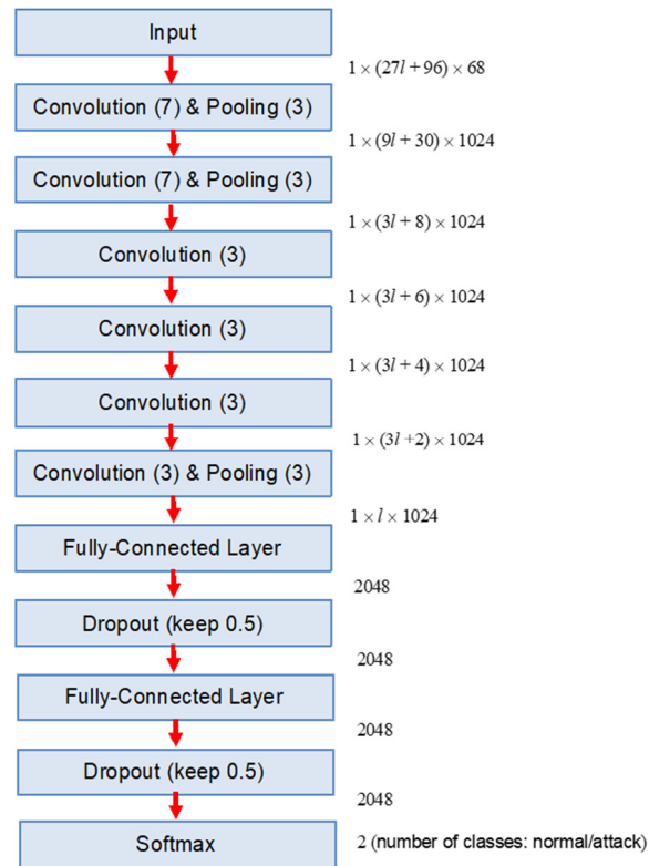
Figure 2: Basic Structure of Cloudbric Deep Learning
